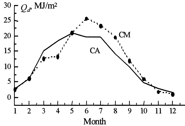
Fig. 6. Dependence of the daily sums of the total radiation on the type of air mass. CA – arctic; CM – midlatitude.
