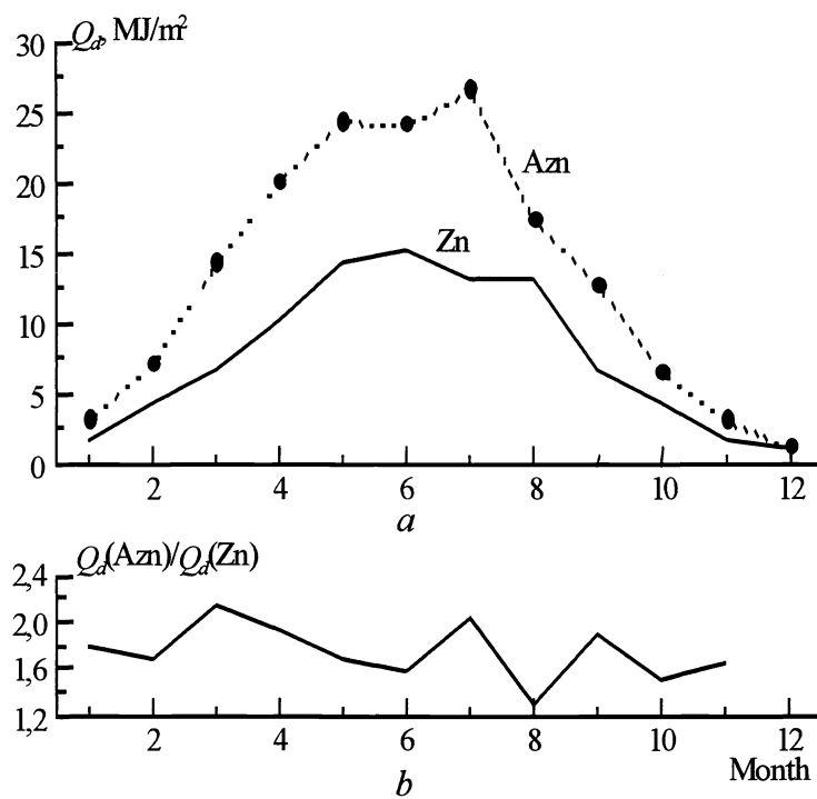
Fig. 5. Dependence of the daily sums of the total radiation on the type of pressure field. Zn – cyclone, Azn – anticyclone.
