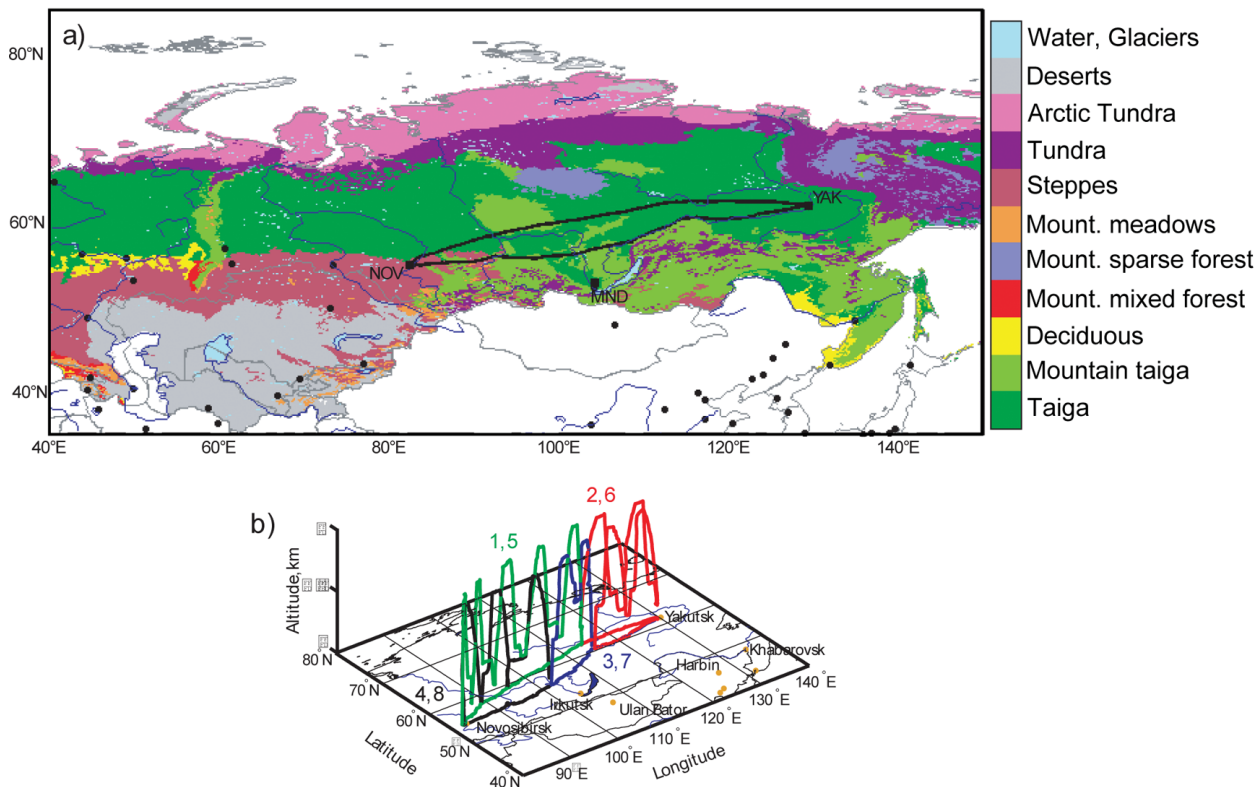
FIG. 2. (a) Flight route and landscape classification. Each campaign follows a similar route, starting from Novosibirsk (NOV) in central Siberia, to the pivot point Yakutsk (YAK), and back to NOV. (b) A campaign is composed of four flights: the first is depicted in green, the second in red, the third in blue, and the fourth in black. The landscape classification is derived from Shvidenko et al. (2007).
