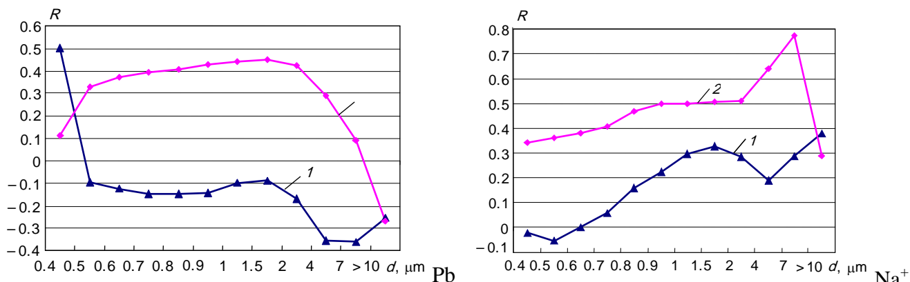
Fig. 6 Correlation curves of two component distribution onto aerosol particles in Tomsk (1) and Kireevsk (2), built by the results of the spring run of measurements, 2001
