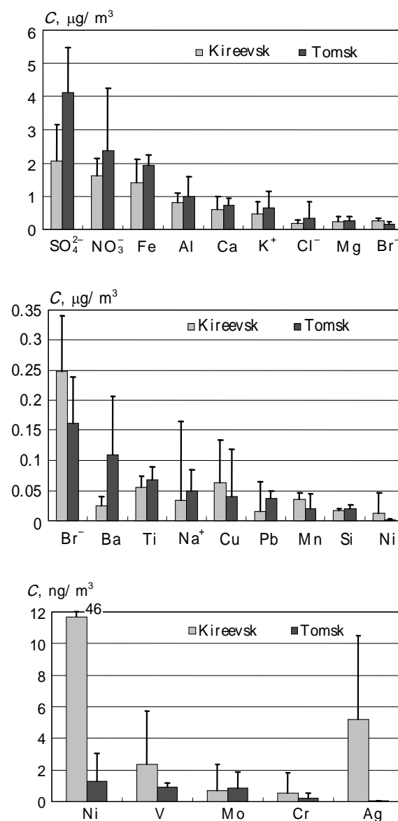
Fig. 2 Mean concentrations of inorganic aerosol components and rms deviations in the fall run of measurements in 1999 ( n = 7 sample pairs).
