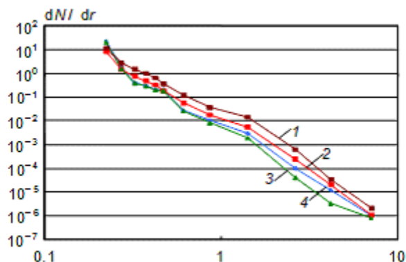
Fig. 4 Mean differential curves of disperse aerosol composition at different sites and different periods of the fall–spring run of synchronous measurements in 2001: Tomsk, April (1) and March (2); Kireevsk, April (3) and March (4).
